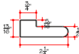
SILL PIECE
